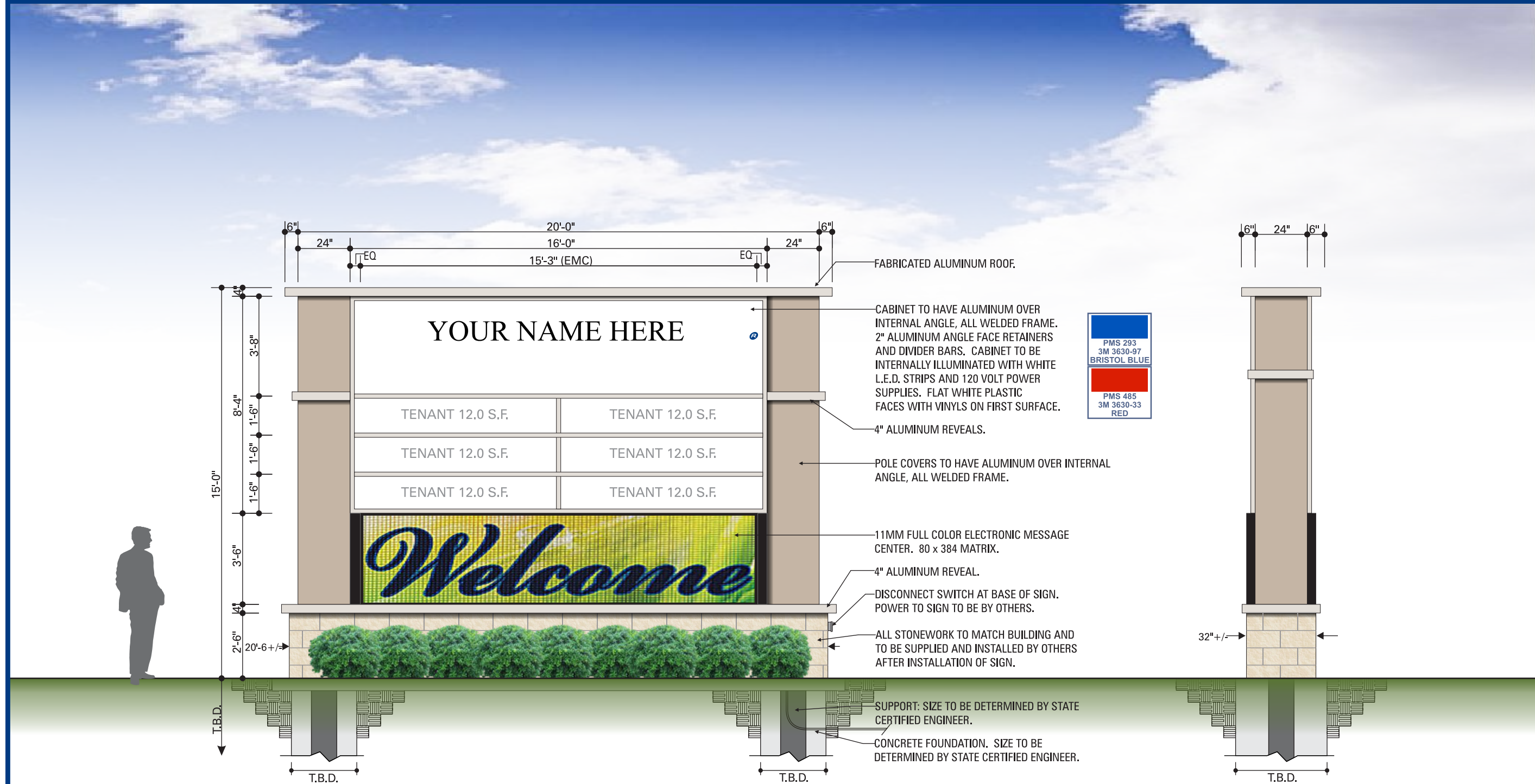
1 FRONT MONUMENT ELEVATION SCALE: 1/4" = 1'-0"
